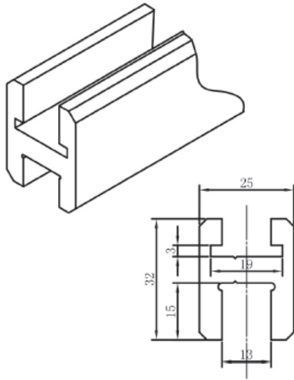
Header extrusion
